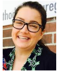
Bragg
